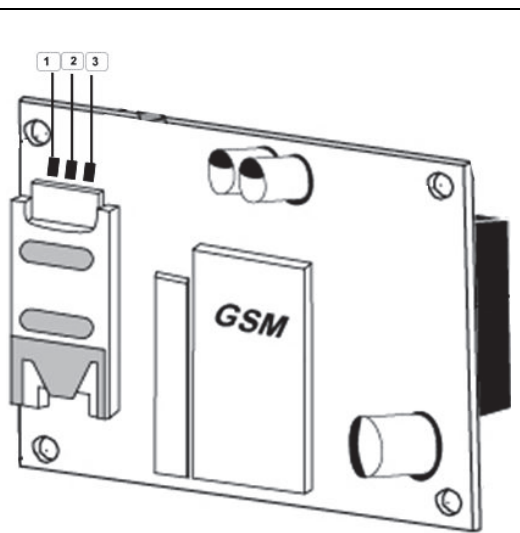
Figure 3: LED's du module GMS
