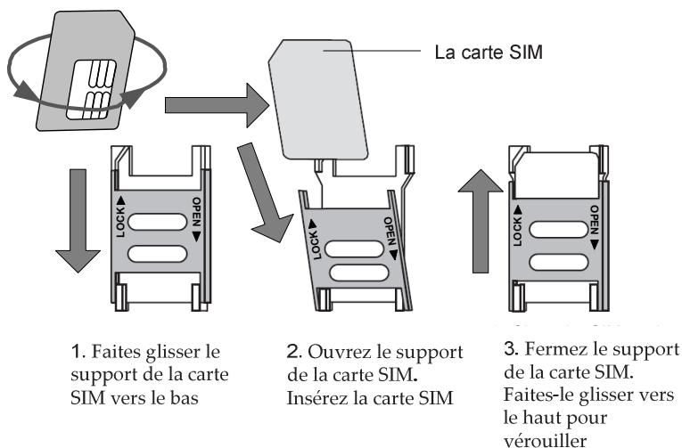
Figure 8: Insertion de la carte SIM
